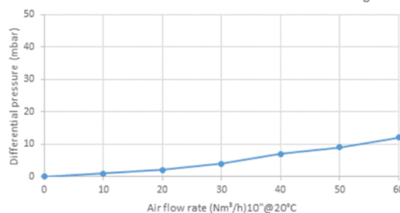
Air Flow Rate: SLF-G-050-10-HSF-S at 0 barg
